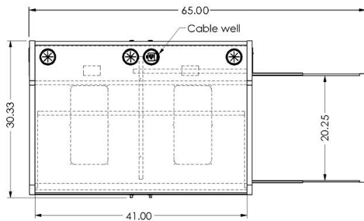
Integrated Cable Well and Grommets
